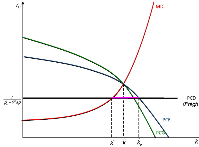
Fig. 1: Intermediation region for a sufficient high pool quality and \rho > \frac{p \cdot m}{\Delta p}
