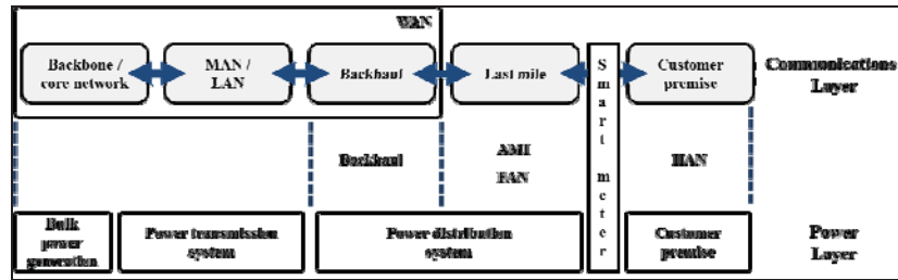
Figure 2: Smart grid communications architecture mapping (based on NIST 2009)
