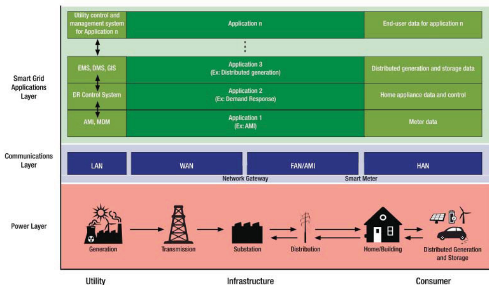
Figure 1: Smart grid architecture (based on Leeds 2009)
