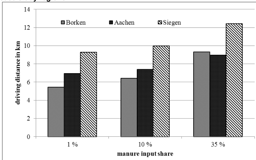
Figure 2: Average driving distances for digestate disposal (500 kW biogas plant) in the three case study regions
