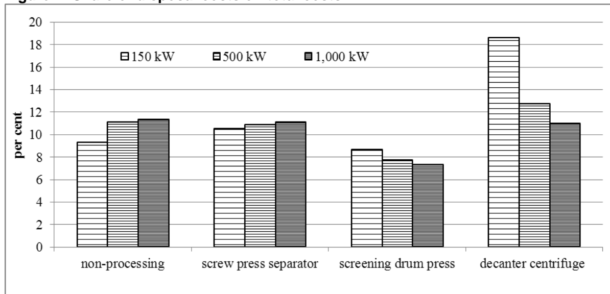
Figure 4: Share of disposal costs on total costs
