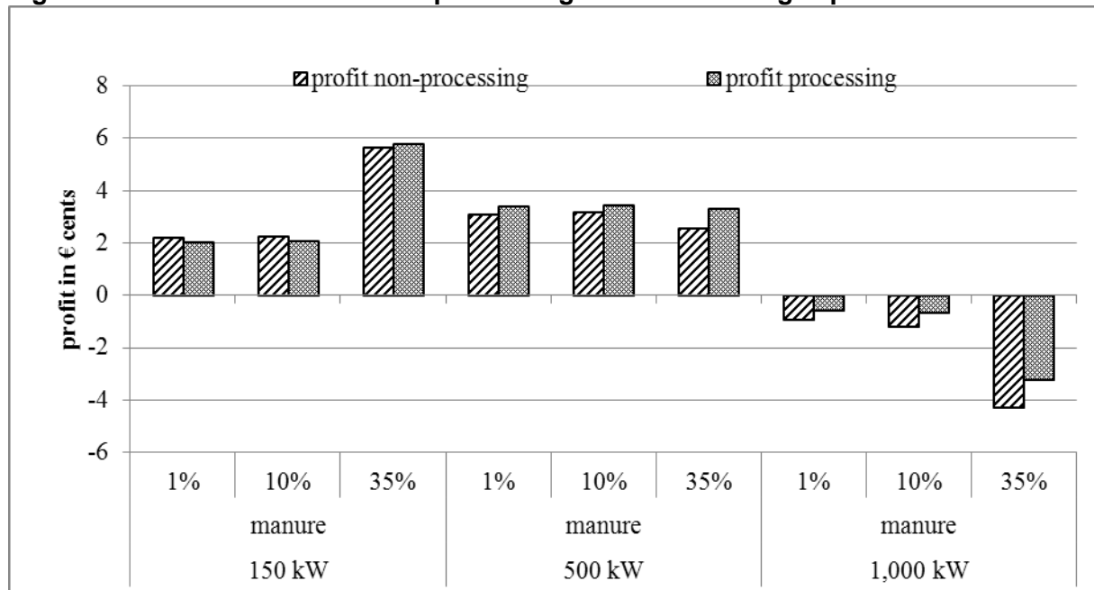
Figure 5: Profits with and without processing for different biogas plant sizes
