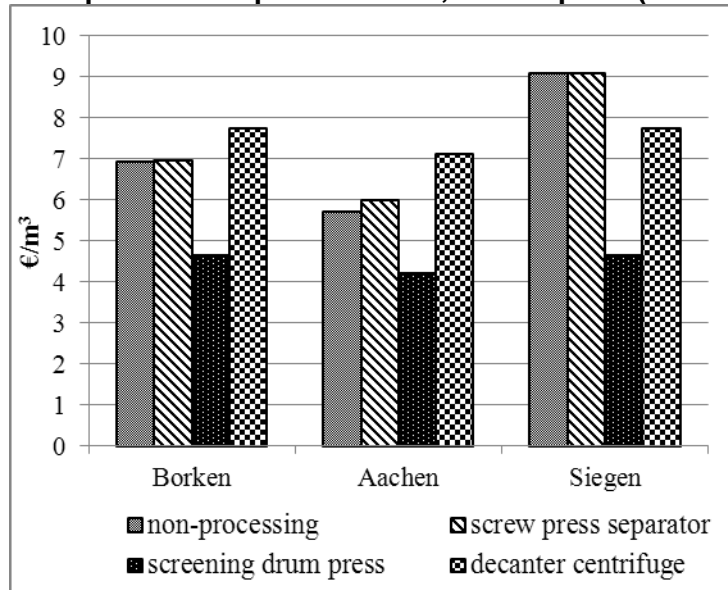
Figure 3: Digestate disposal costs per m 3 for a 1,000 kW plant (10% manure input)
