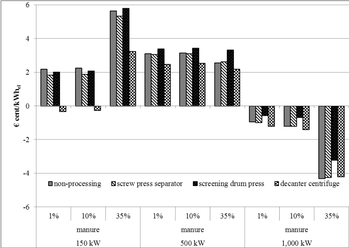
Figure 6: Total profits for different plant sizes and manure shares by processing technique
