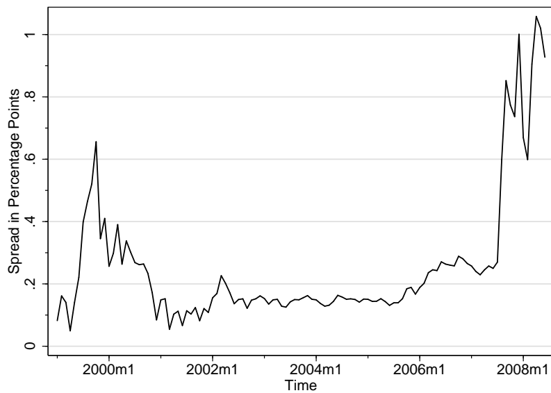
Figure 4: Euribor-Bubill Spread
