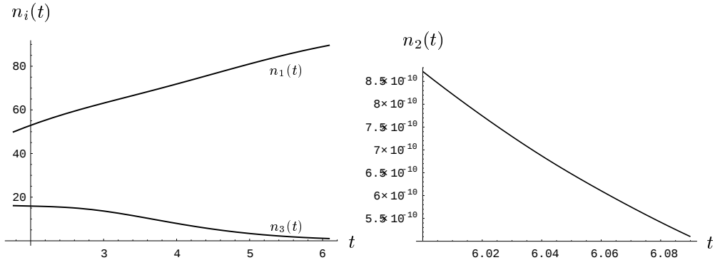
Figure 4: Prey extinction
