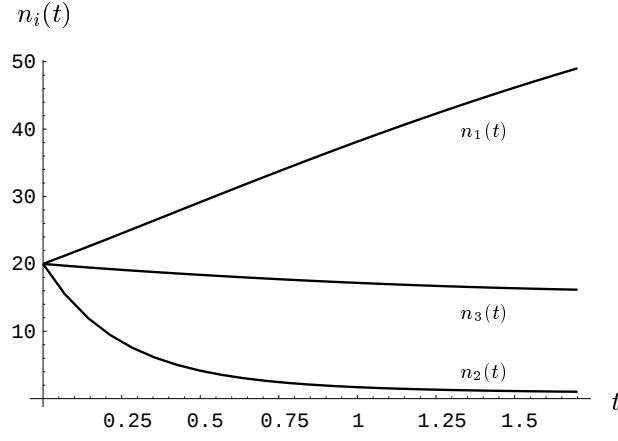
Figure 4: Prey extinction
