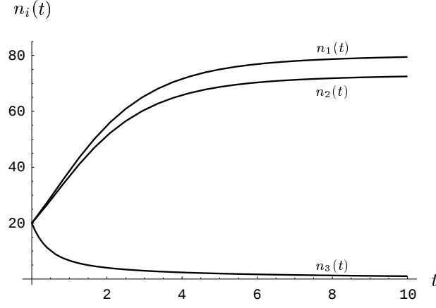
Figure 2: Predator extinction
