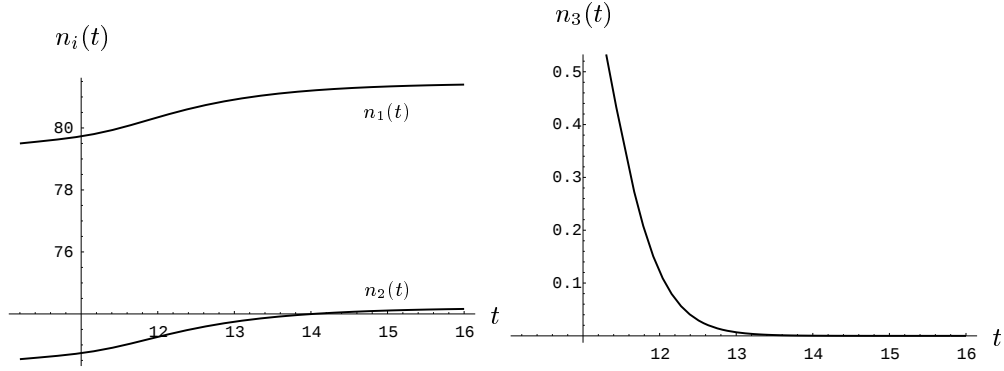
Figure 2: Predator extinction
