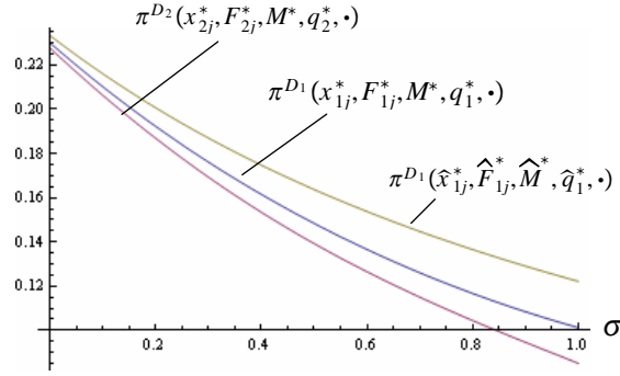
Figure 4 b: Downstream Profits for N = 10
