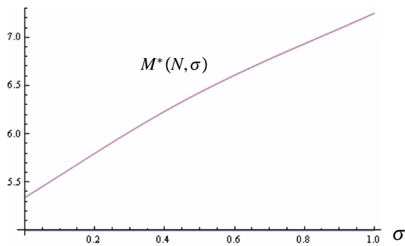
Figure 2: M^*(N, \sigma) for N = 10
