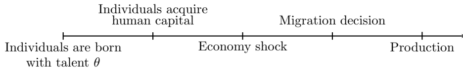
Figure 2: The Timeline
