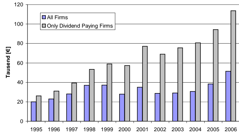
Figure 6: Mean Dividend
