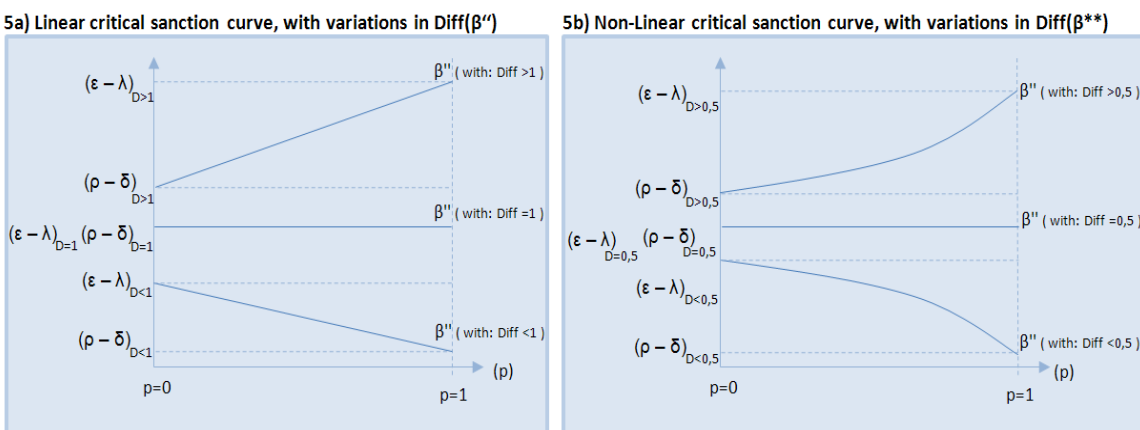
Figure 5: Linear and non-linear critical sanction curve, with variations in \text{Diff}(\beta'') and \text{Diff}(\beta''^*)
