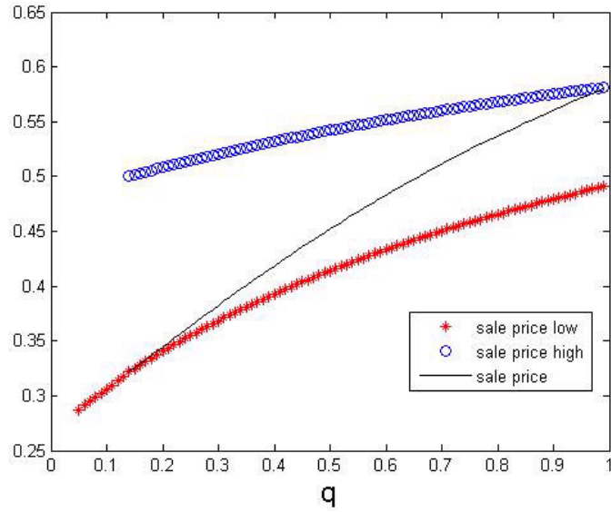
Figure 7: Average selling price and the fraction of type-H sellers, \theta = 2 , s = 0.5
