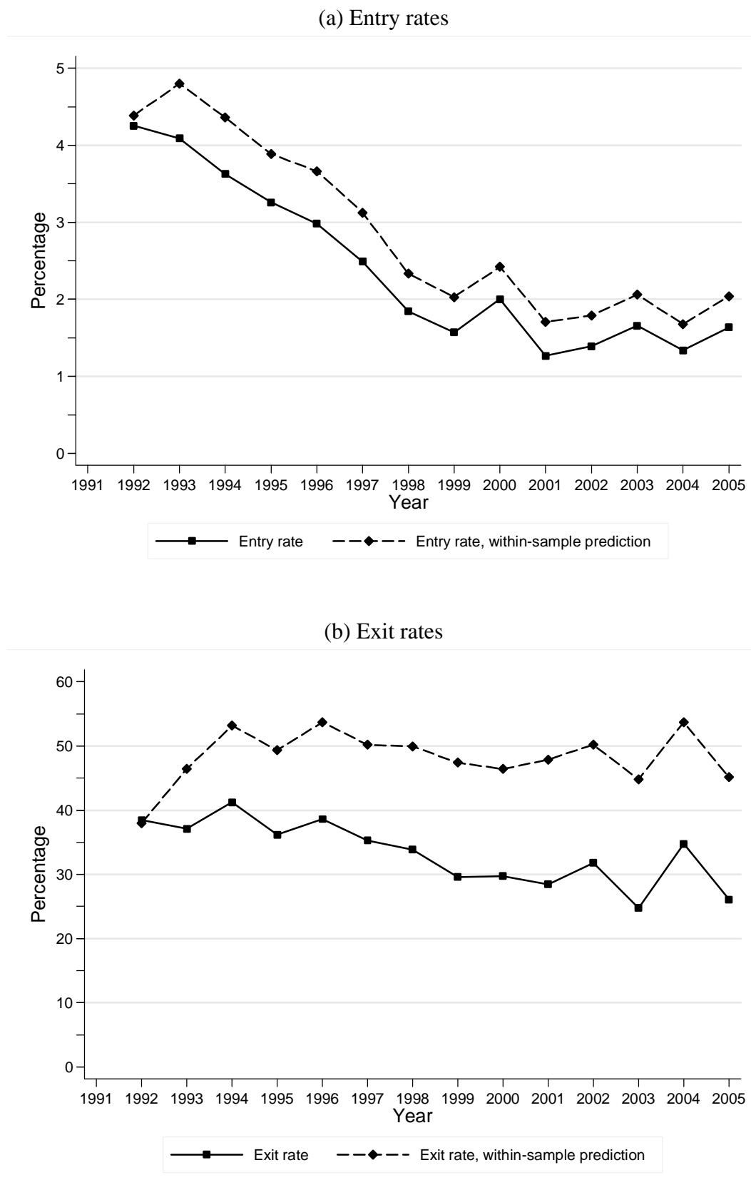
Figure 3. Within-sample predictions of SA transition rates compared to aggregate transition rates
