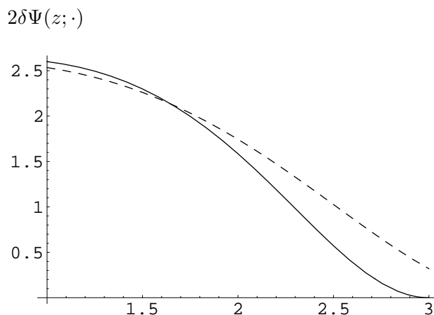
Figure 5: Thresholds may decrease in MPS. We have graphed 2\delta\Psi(z; \cdot) with \delta = 0.65 for two different uniform distributions. The solid line is drawn for support [1, 3] , while the dashed line is drawn for support [0.5, 3.5] . For low values of z the MPS causes a decrease in \Psi(z; \cdot) .
