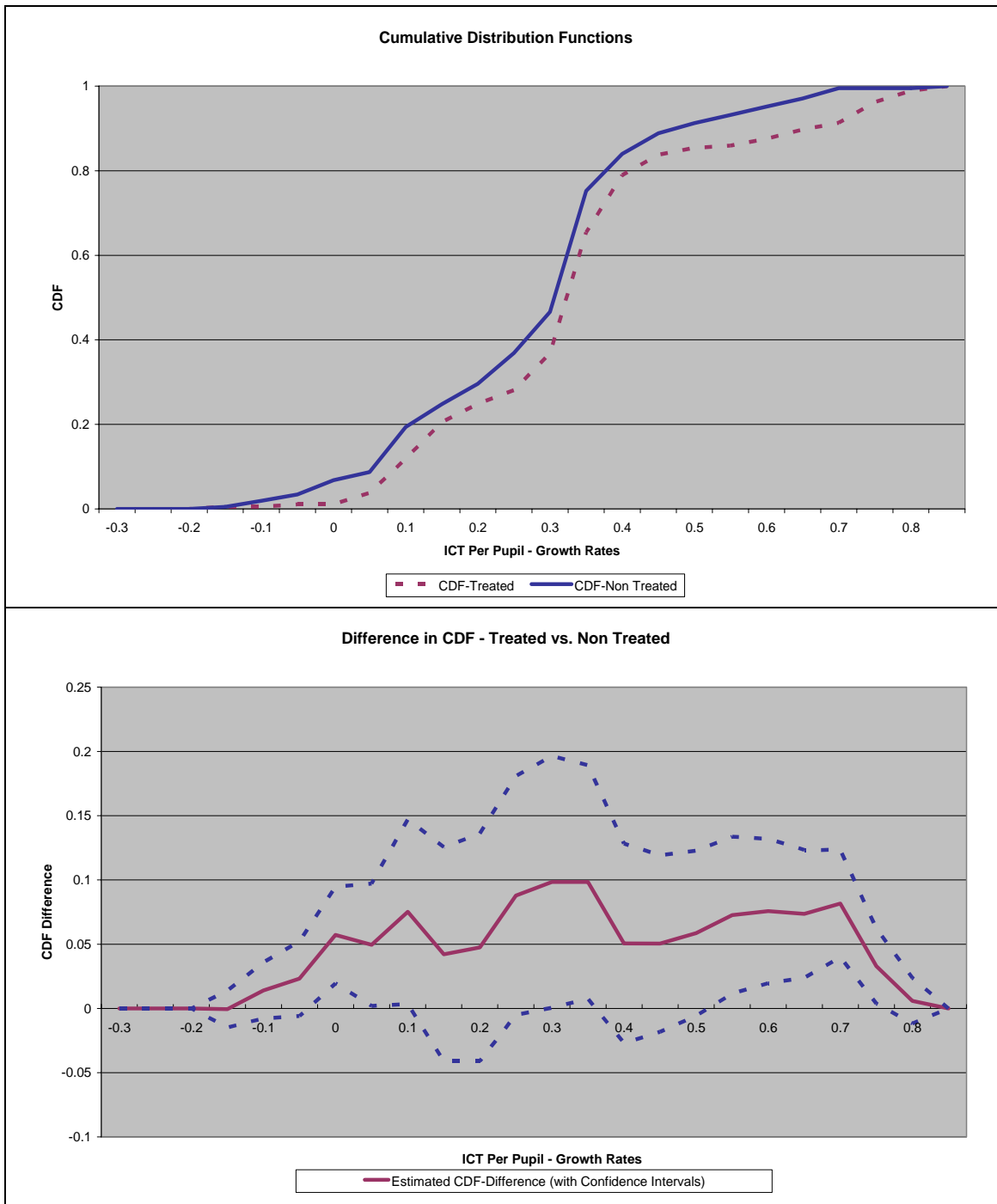
Figure 6: Impact of the Instrument and Average Causal Response (ACR) Interpretation.
