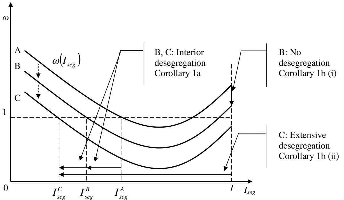
Figure 6: The effects of \chi on equilibrium segregation
