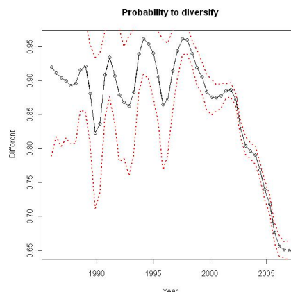
Figure 4: Estimated probability to diversify over time
