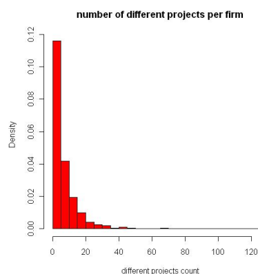
Figure 2: Total number of different projects per firm
