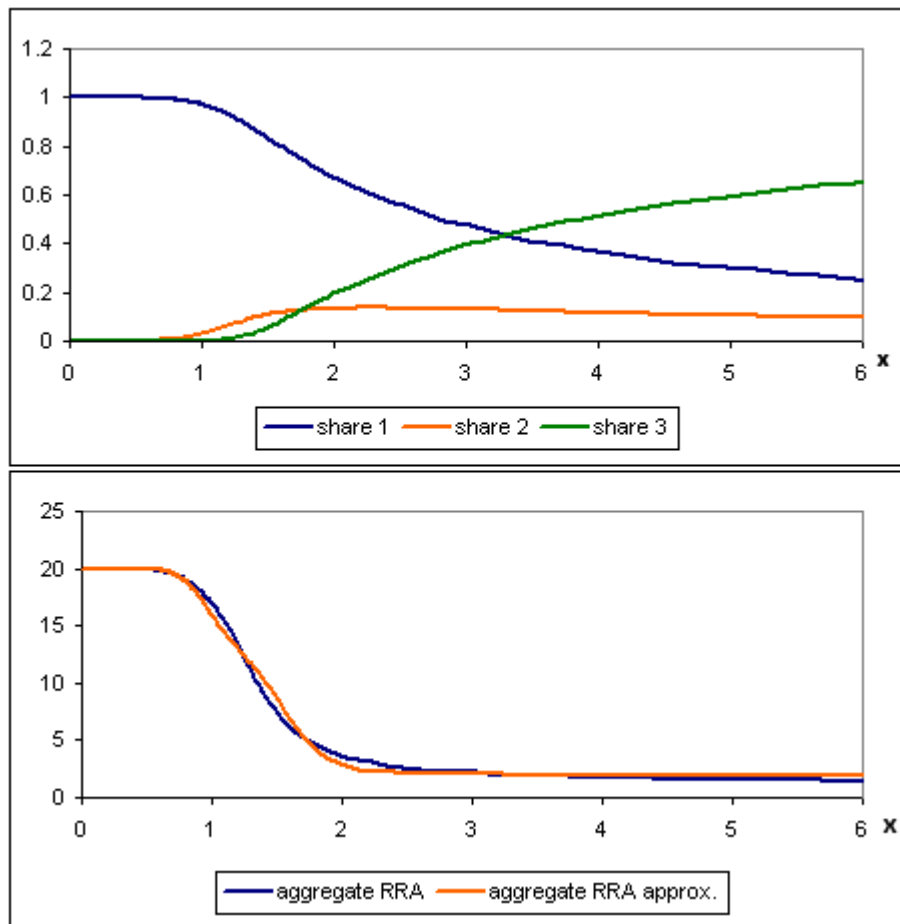
Figure 2: (\gamma) = (20; 3; 1) and 1/\lambda = (10^{-3}; 20; 1)
