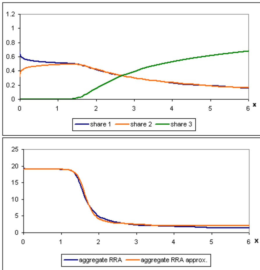
Figure 3: (\gamma) = (20; 18; 1) and 1/\lambda = (10; 6; 1)
