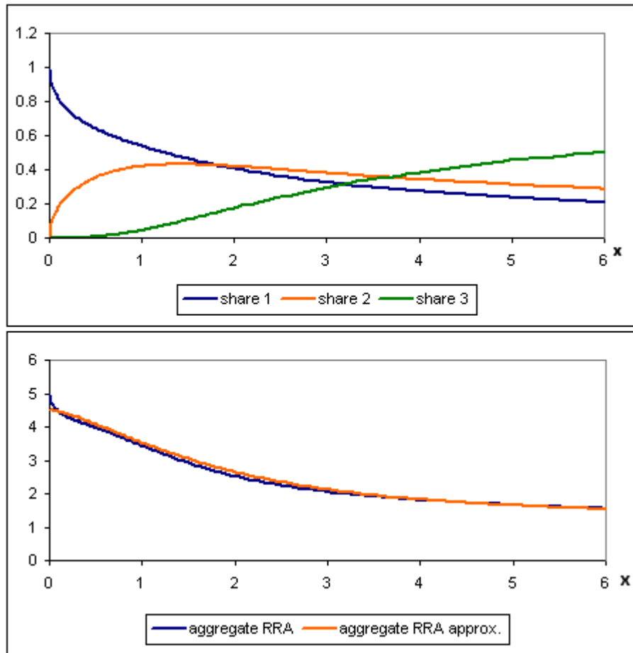
Figure 1: (\gamma) = (5; 3; 1) and 1/\lambda = (1; 3/5; 1)
