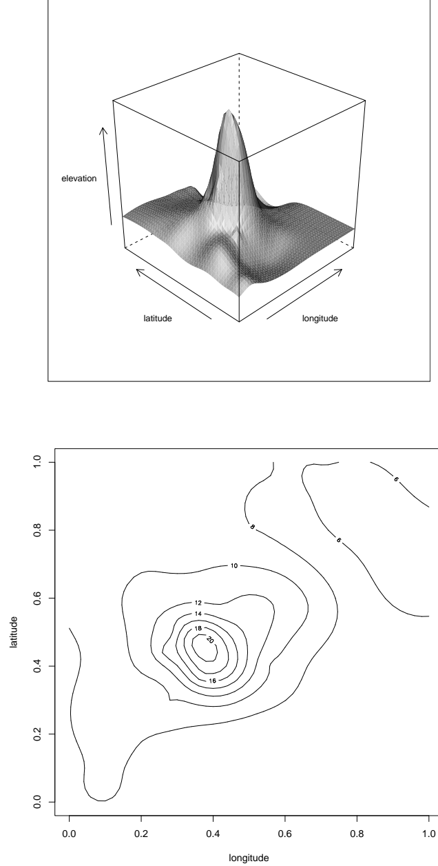
Figure 9. Noshiro data: Fit with gMDL-stopped L2KnotSmooth, surface (upper panel) and contour plot (lower panel)
