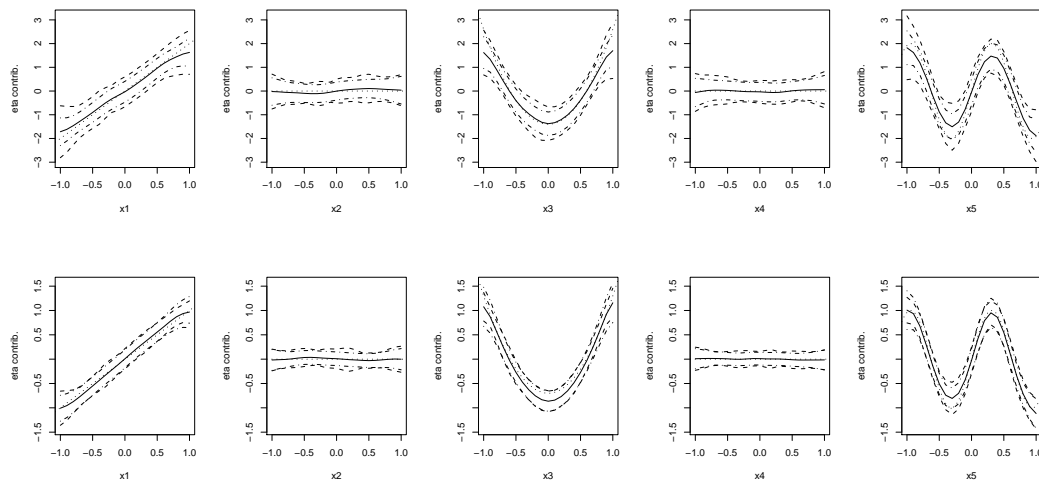
Figure 4: Mean empirical (broken lines) and estimated (dash-dotted lines) confidence bands for 50 fits to data from a binary response (upper panels) and a Poisson response model (lower panels). The solid lines indicate the estimates and the dotted lines the true functions.
