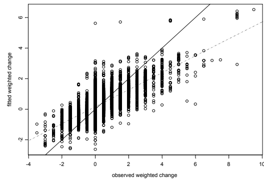
FIGURE 7. Plot of observed against fitted values (dashed line: linear regression line of the scatter plot; full line: the diagonal)
