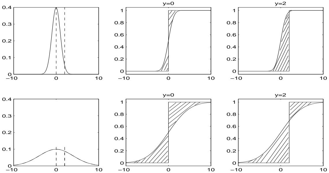
Figure 1: Pdf (left column with y = 0, 2 indicated as dashed lines) and cdf of a normal distribution with mean 0 and standard deviation 1 (first row) and 2 (second row), respectively. The differences between the cdf and the empirical cdf for two observations y = 0 (middle) and y = 2 (right) are indicated as shaded regions.
