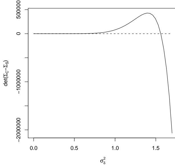
Figure 1: The determinant of \Sigma_C - \Sigma_S as a function of \sigma_\delta^2
