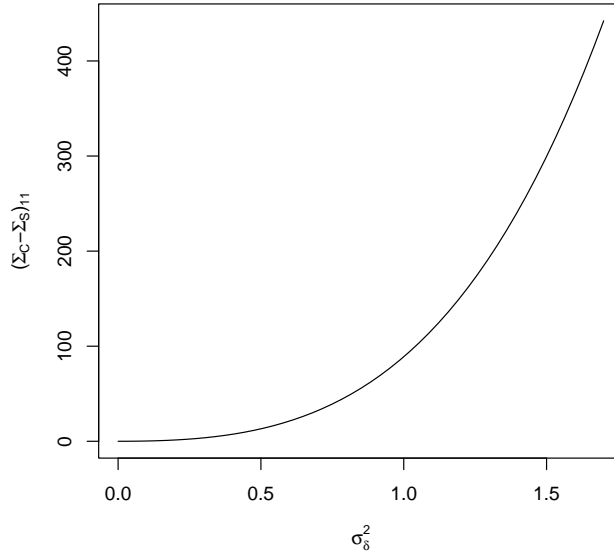
Figure 2: The first diagonal element of \Sigma_C - \Sigma_S as a function of \sigma_\delta^2
