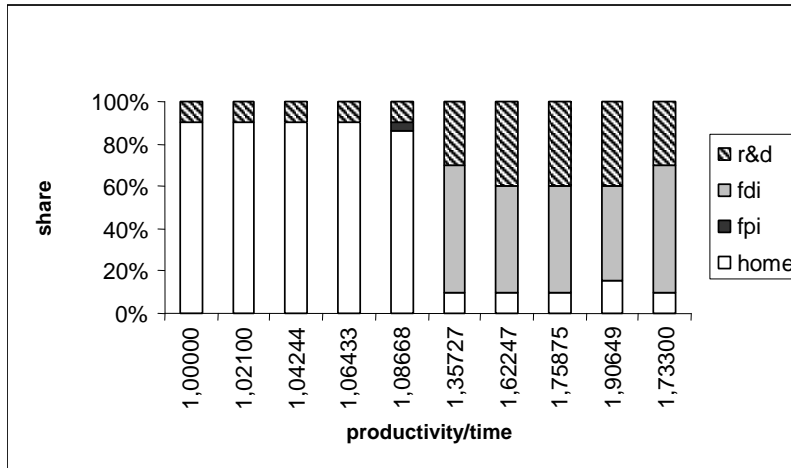
Figure 1: Isolated investmentshares of all four possible investments depend on time and domestic productivity. R&D success probability \lambda = 0.3 .
