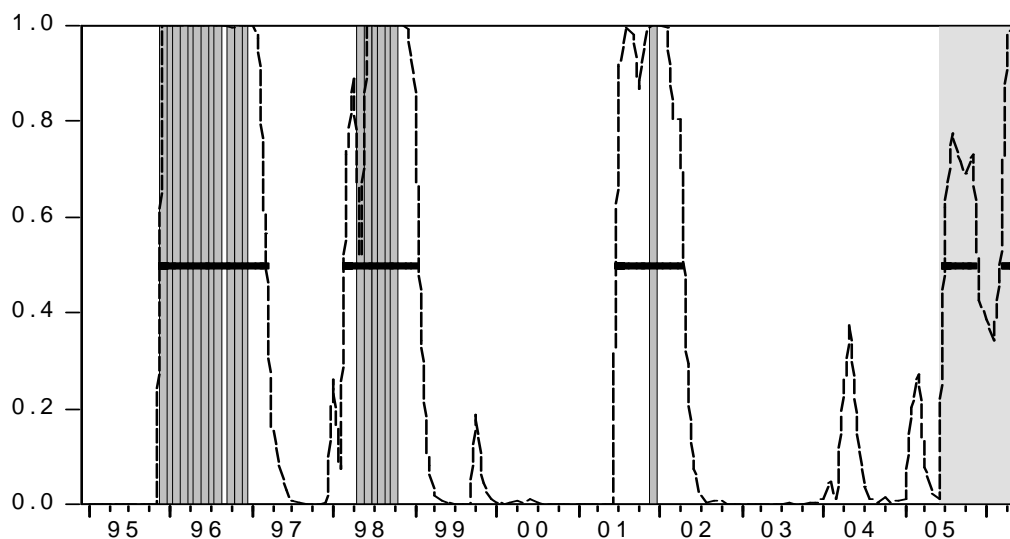
Figure 7: Markov-switching Forecast
