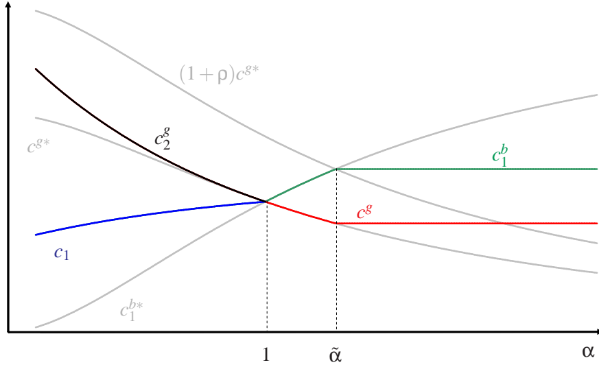
Figure 3: Second-best consumption
