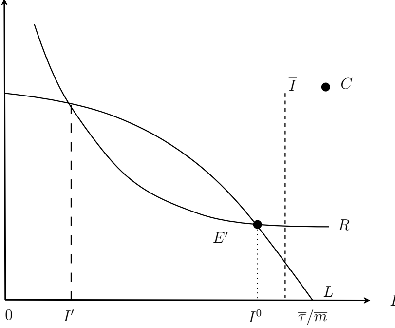
Figure B: 1 \leq \rho(1 - \varphi) .
