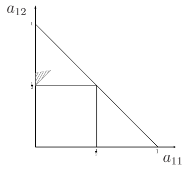
Feasible set \mathcal{S}_{\mathcal{B}_6}
