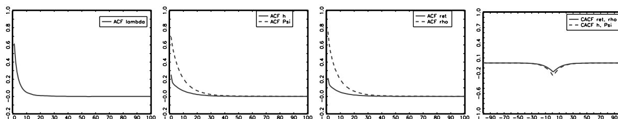
Figure 3: \omega = (0, 0) , \alpha_0^{13} = 0 , A_1 = (0.1 \ 0, 0 \ 0.1) , B_1 = (0.1 \ 0, 0 \ 0.1) , a = 0.9 , \delta_1 = 0.3 , \delta_3 = -0.3 .
