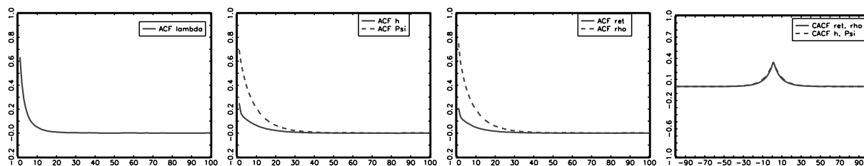
Figure 2: \omega = (0, 0) , \alpha_0^{13} = 0 , A_1 = (0.1 \ 0, 0 \ 0.1) , B_1 = (0.1 \ 0, 0 \ 0.1) , a = 0.9 , \delta_1 = \delta_3 = 0.3 .
