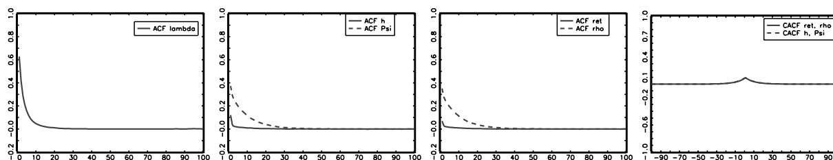
Figure 1: \omega = (0, 0) , \alpha_0^{13} = 0 , A_1 = (0.1 \ 0, 0 \ 0.1) , B_1 = (0.1 \ 0, 0 \ 0.1) , a = 0.9 , \delta_1 = \delta_3 = 0.1 .
