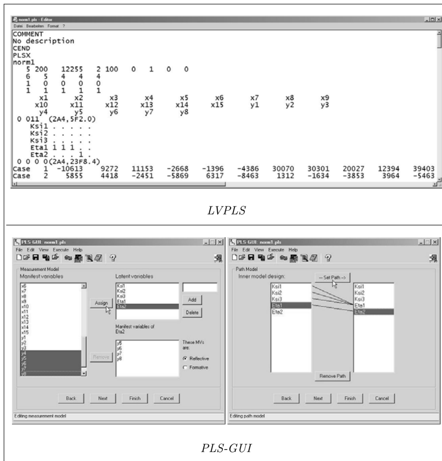
Fig. 1. Specification of Path Models in PLS Software: LVPLS , PLS-GUI
