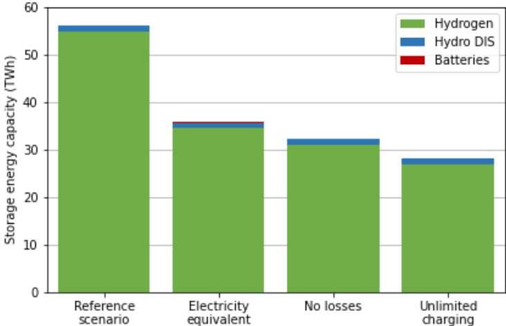
Figure 5: Storage energy capacity in the reference scenario and for the hypothetical cases of loss-free storage and, in addition, unlimited charging capacity
