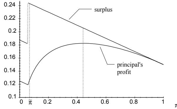
Figure 1. Imperfect surveillance.
