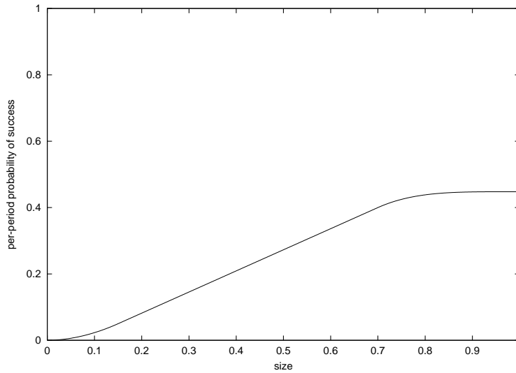
Figure 7: Per-period probability of success as a function of firm size (market share [%])
