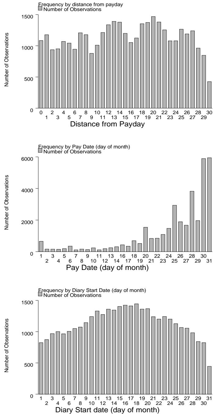
Figure 3: Descriptive Statistics
