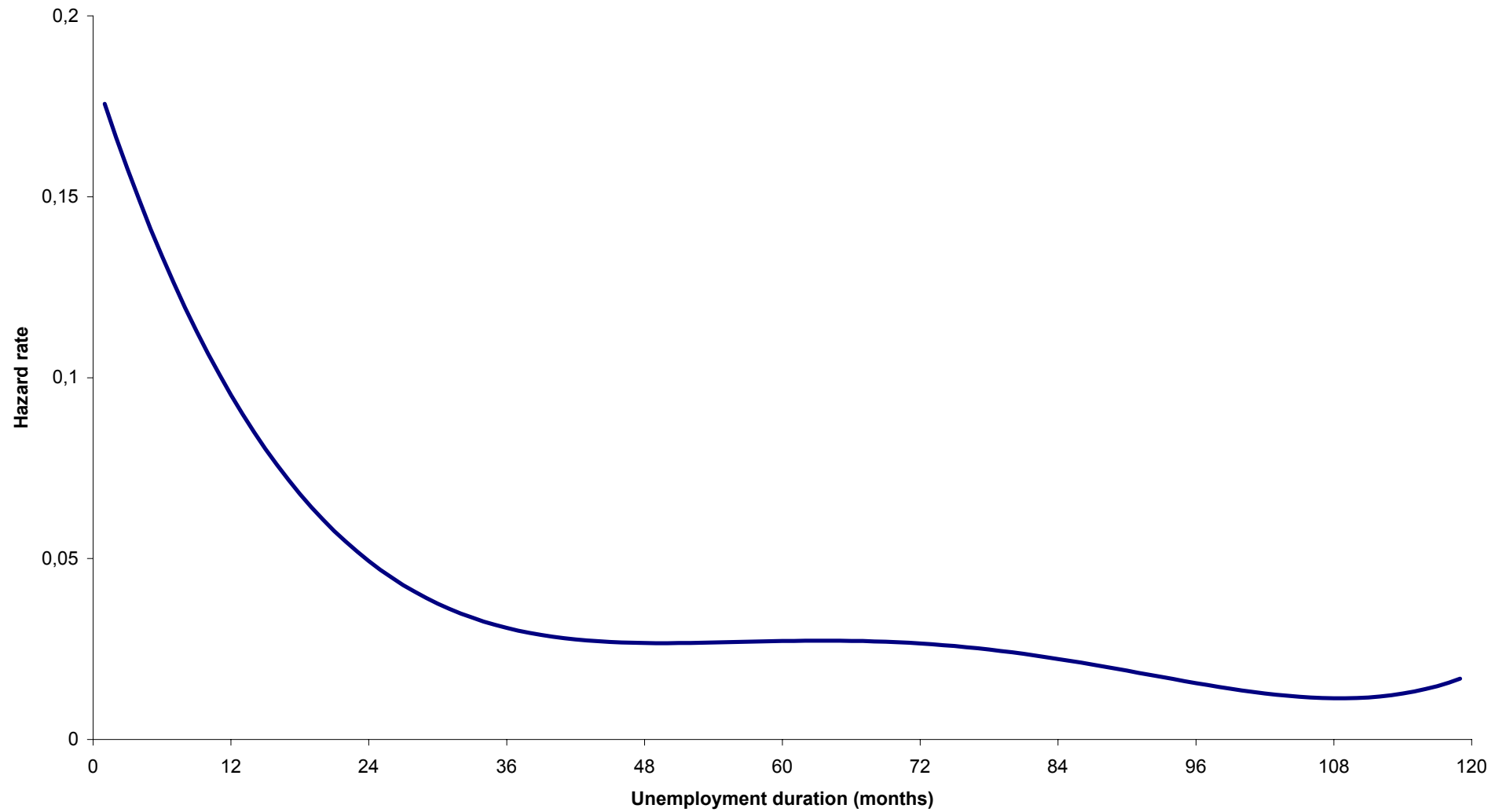
Figure 1: Baseline Hazard Function (4th degree polynomial function)
