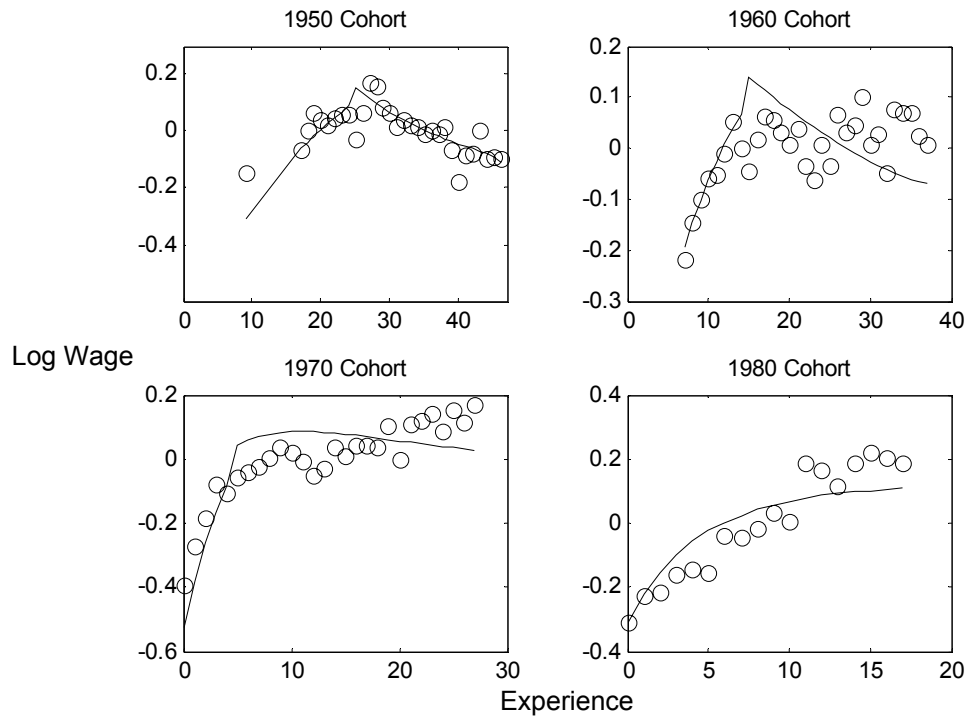
Figure 4. Actual and predicted lifecycle earnings by cohort.
