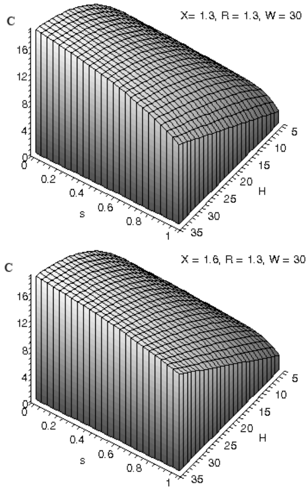
Figure 3: Plot of C_t against s_t and H_t ( X_t = 1.3 and X_t = 1.6, W_{t-1} = 30, E[R]_{t+1} = 1.3 )
