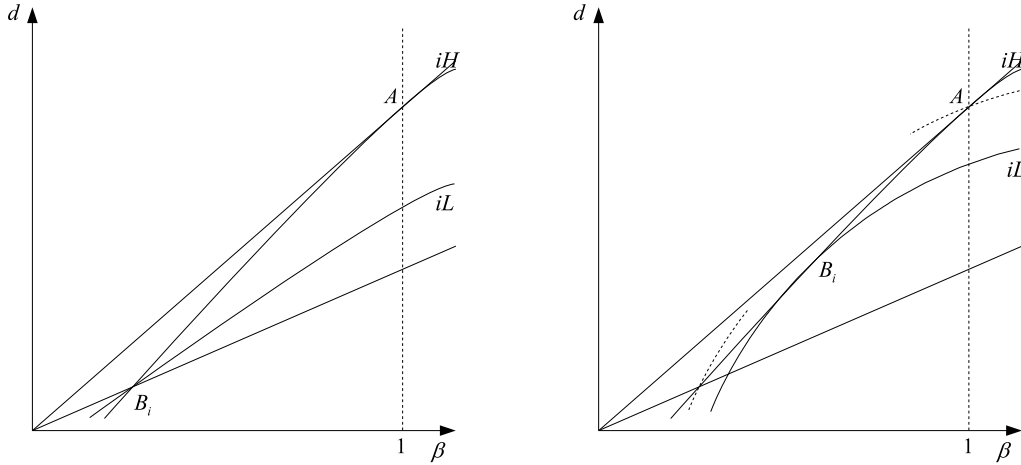
Figure 1: Observable Productivities
