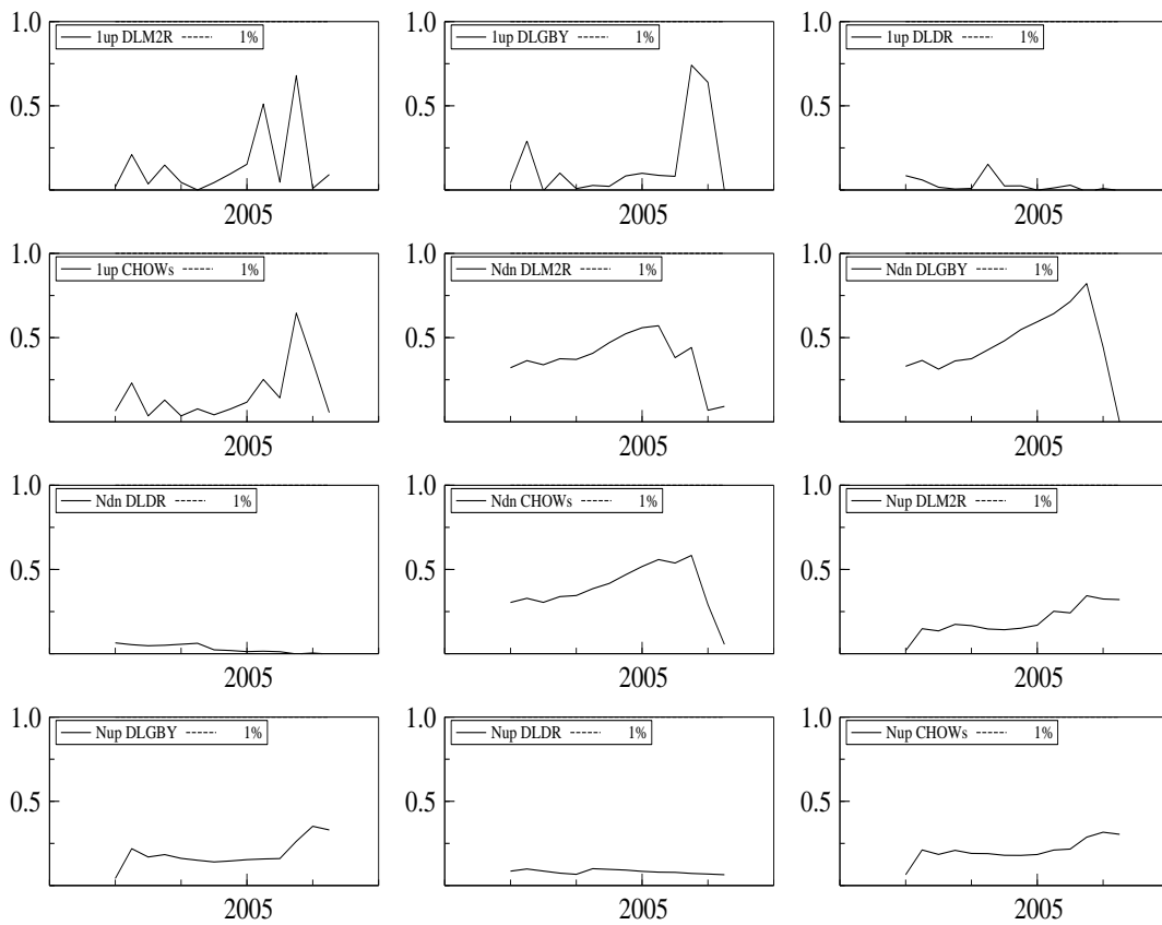
Figure 6: VECM: Chow test statistics, scaled by the 1% critical values
