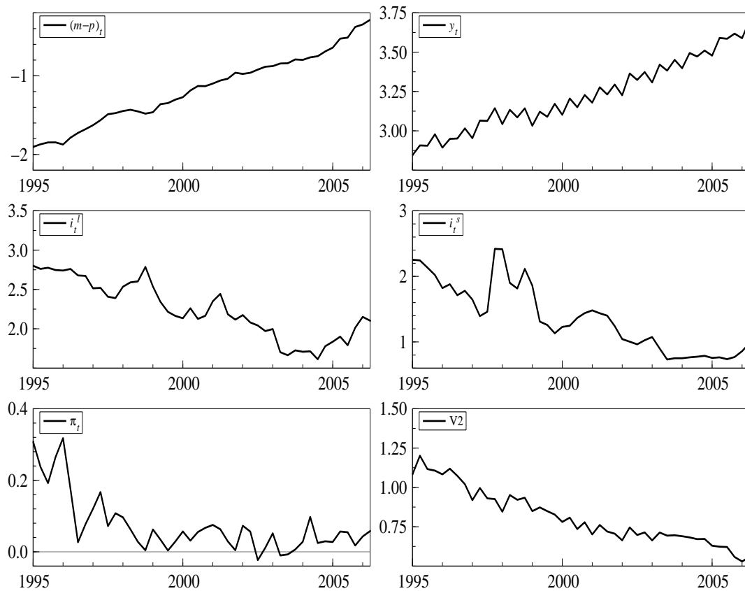
Figure 1: Data: 1995:I - 2006:II
