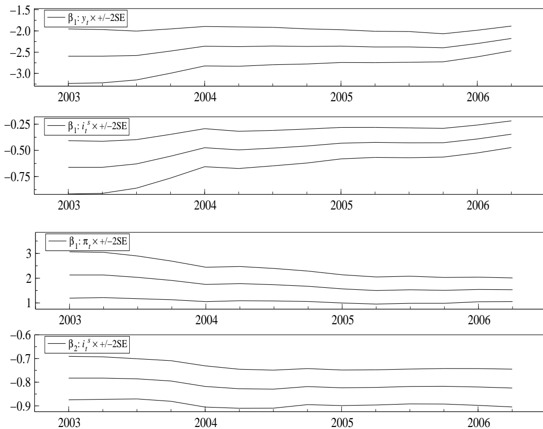
Figure 4: VAR model: Recursively estimated coefficients of the identified cointegrating vectors \beta_1 and \beta_2
