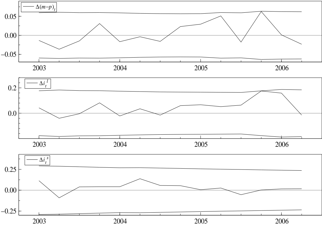
Figure 7: VECM: One-step ahead residuals
