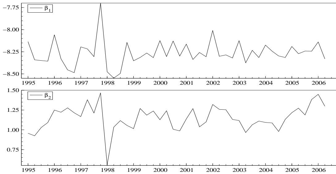
Figure 3: VAR model: Cointegrating vectors
