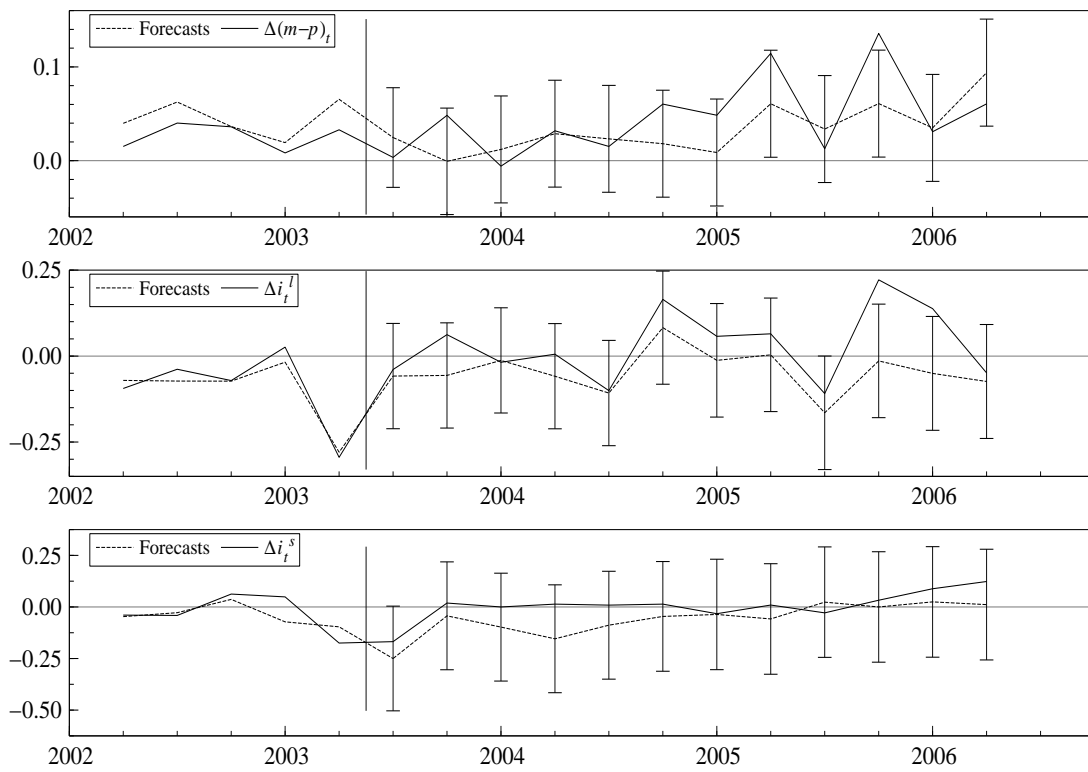
Figure 8: VECM: 1-step ahead ex post forecasts
