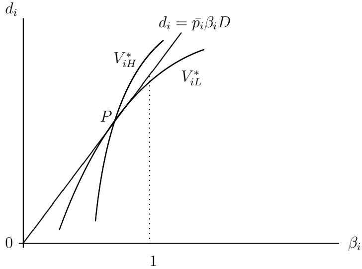
Figure 2: Wilson pooling equilibrium ( \alpha = 0 )
