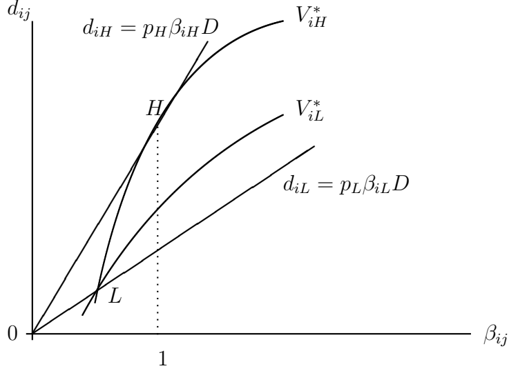
Figure 1: Rothschild-Stiglitz separating equilibrium ( \alpha = 0 )
