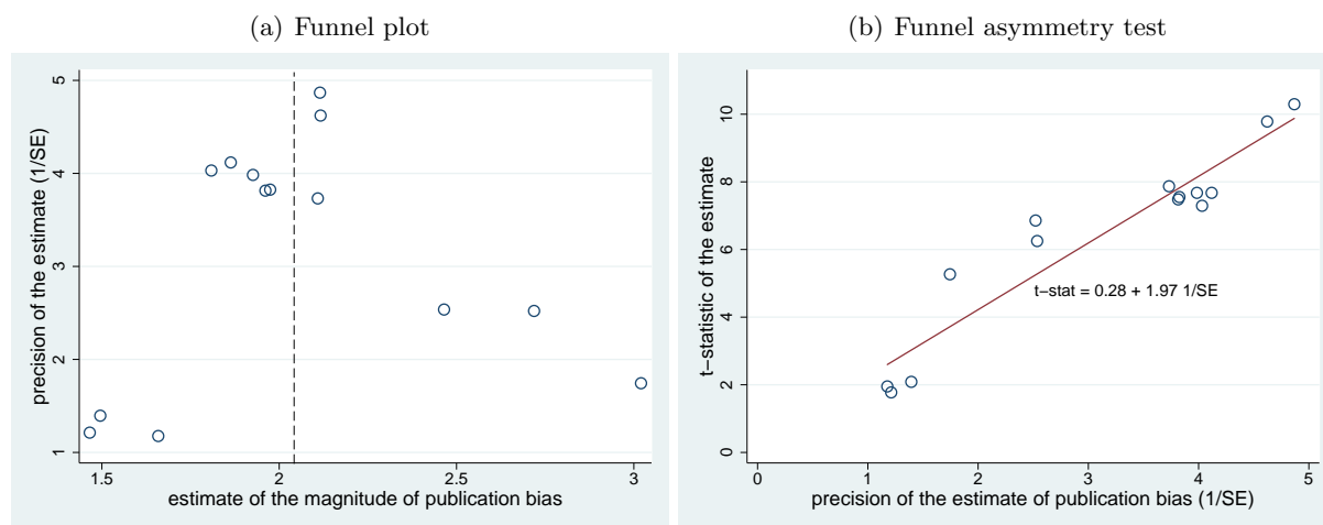
Figure 3: Publication bias in the estimates of the bias?
