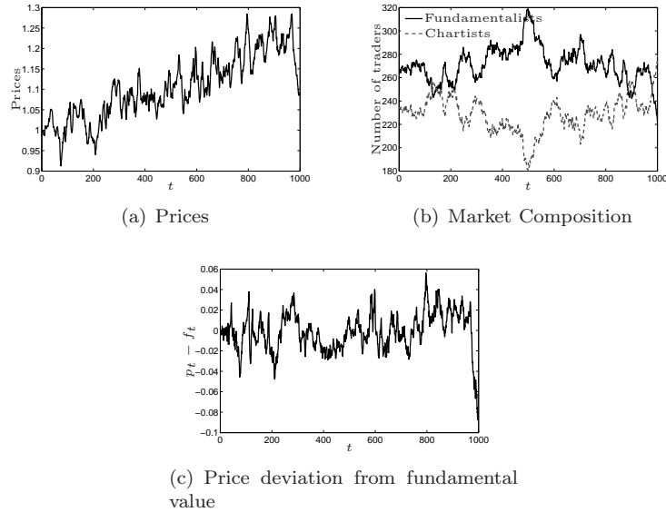
Figure 3: Dynamics in an exemplary simulation.
